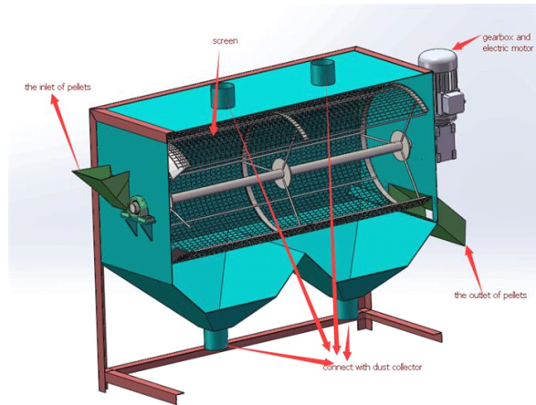
Horizontal pellet cooler inner structure
